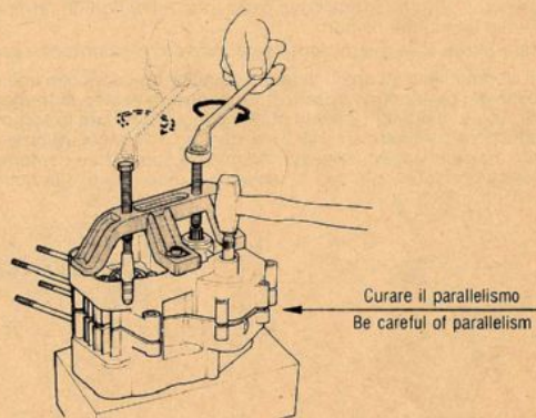
FIG. 24 Apertura semicarteri Half-crankcase opening
