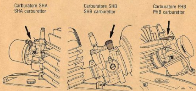
FIG. 2 Starter Choke lever
