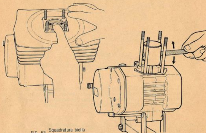
FIG. 53 Squadratura biella Connecting rod squaring
