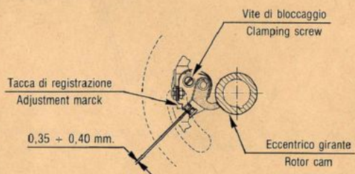
FIG. 6 Contatti volano Flywheel magneto contacts
