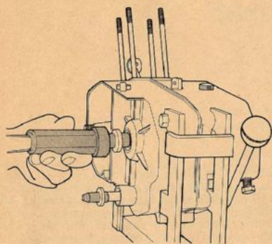
FIG. 45 Montaggio paraoli Oil seals assembly
