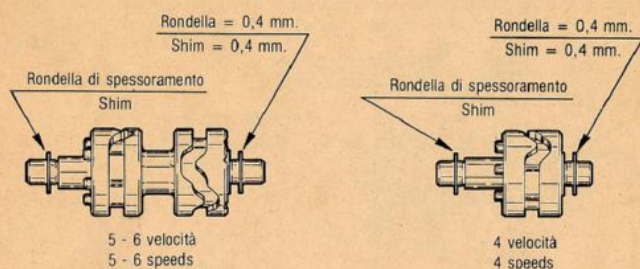
FIG. 31 Desmodromico Gear-box cam
